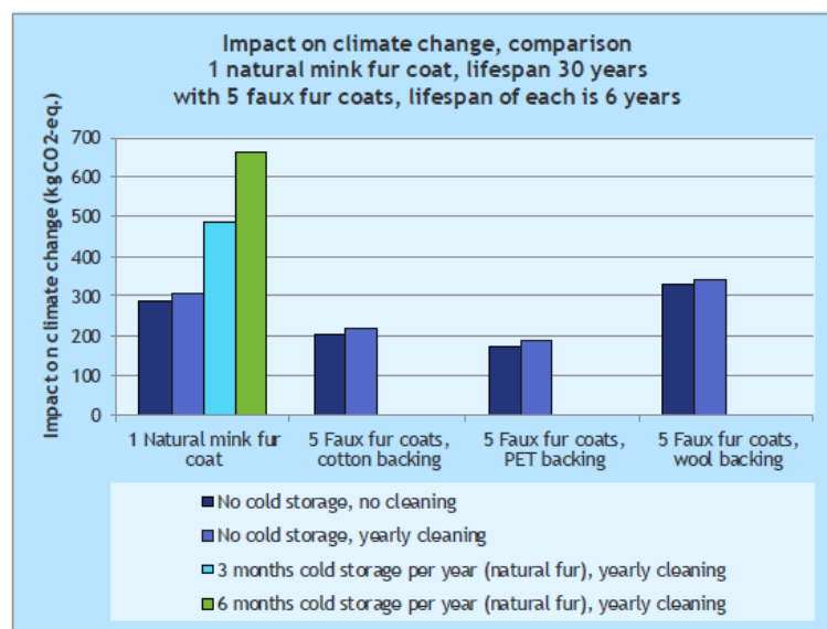
Figure 7 Impact on climate change, CE Delft inventory, lifespan scenario by DSS, 2011
